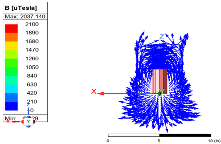
Figure 3.4: Magnetic field in XZ plane
