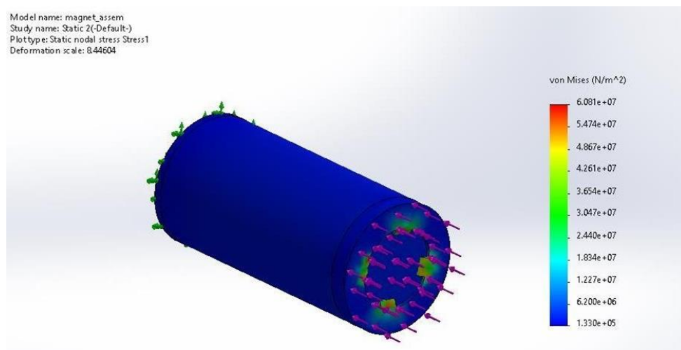
Figure 3.7: Magnet stress plot
