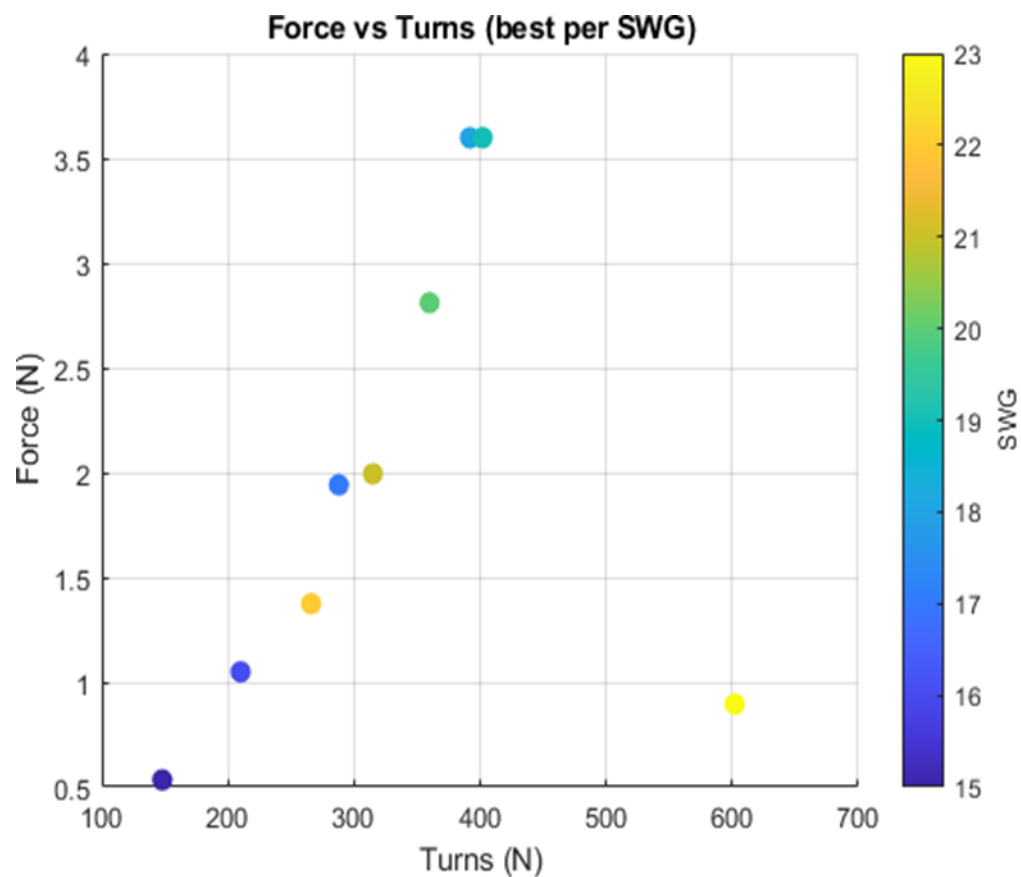
Figure 3.1: Force vs Turns
