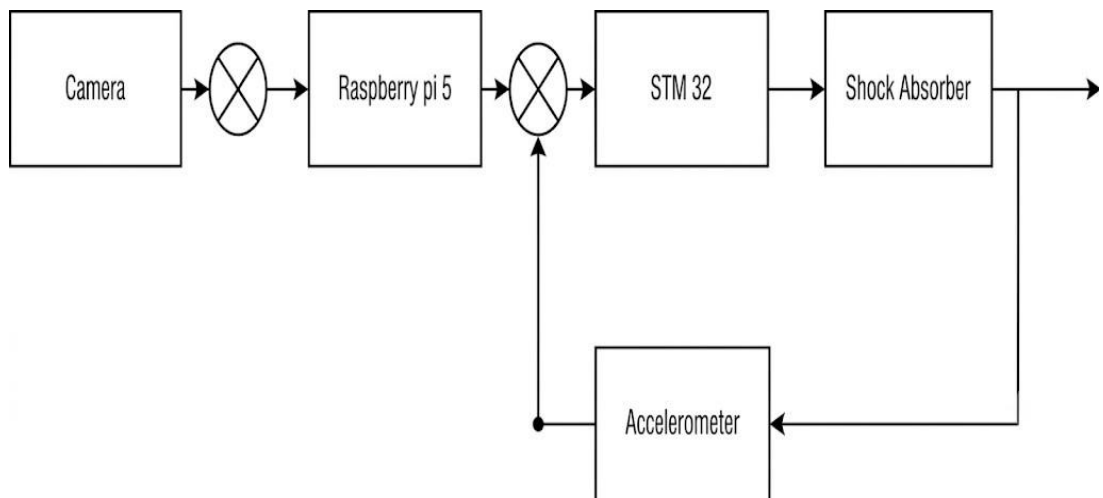
Figure 2.2: Block diagram.
