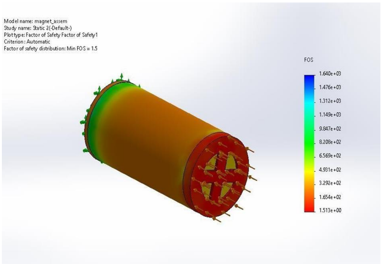
Figure 3.8: Magnet factor of safety
