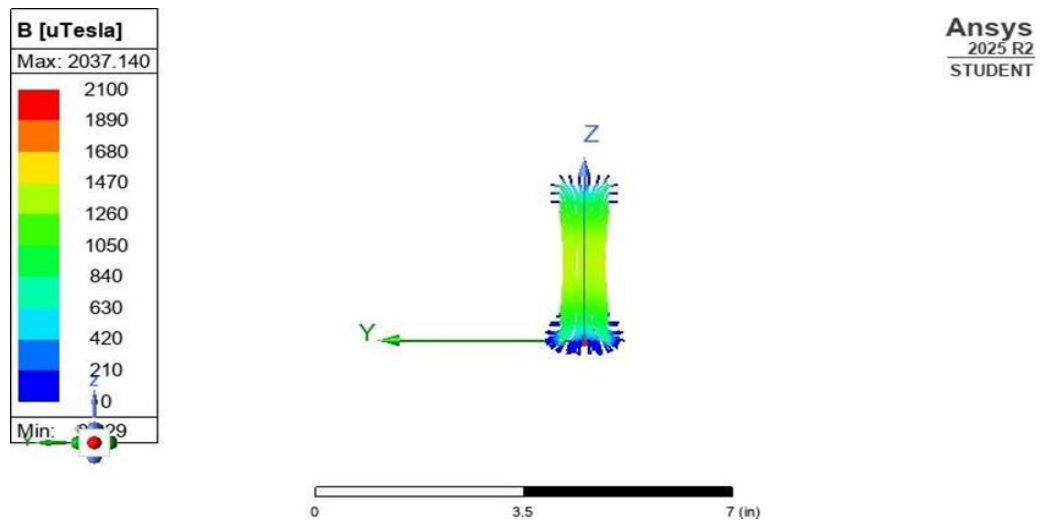
Figure 3.3: Magnetic field in YZ plane
